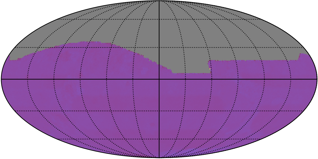
too_elab_heavy_r32_d2_griz_v3.4_10yrs All sky: Normalized Proper Motion Uncert @ 20.5
