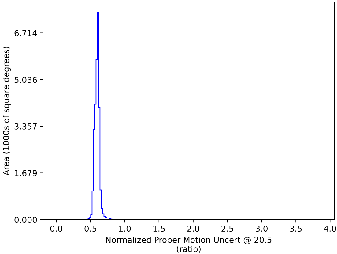
too_elab_heavy_r32_d2_griz_v3.4_10yrs All sky: Normalized Proper Motion Uncert @ 20.5
