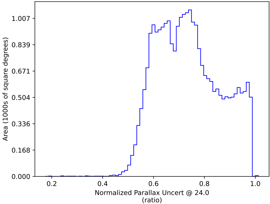
too_elab_heavy_r32_d2_griz_v3.4_10yrs All sky: Normalized Parallax Uncert @ 24.0
