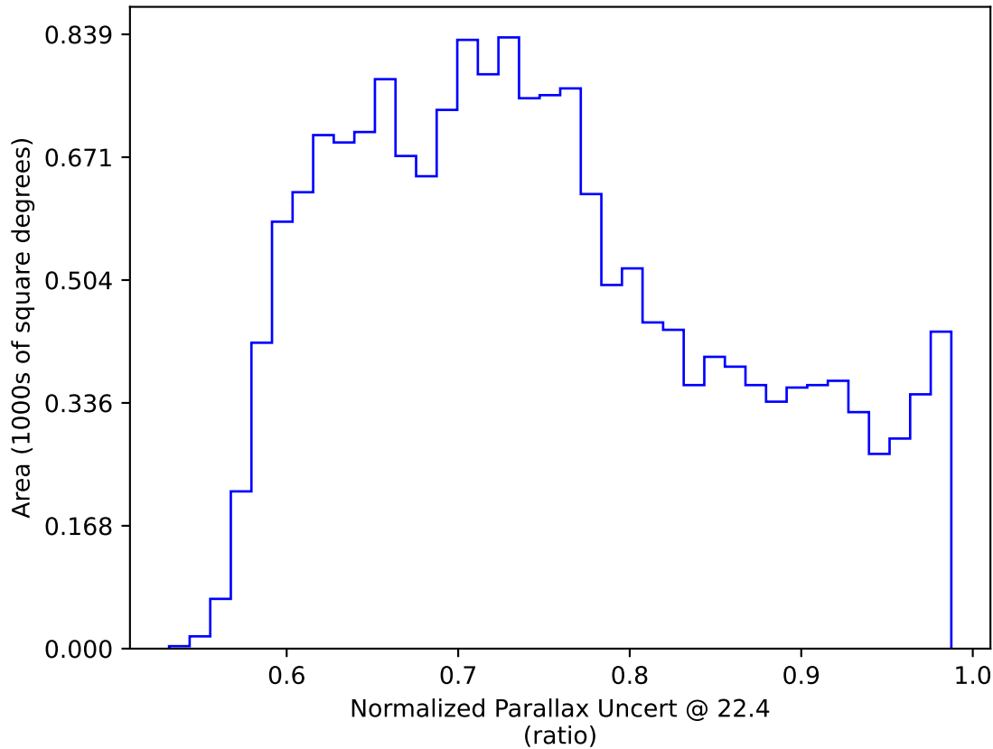
too_elab_heavy_r32_d2_griz_v3.4_10yrs WFD: Normalized Parallax Uncert @ 22.4
