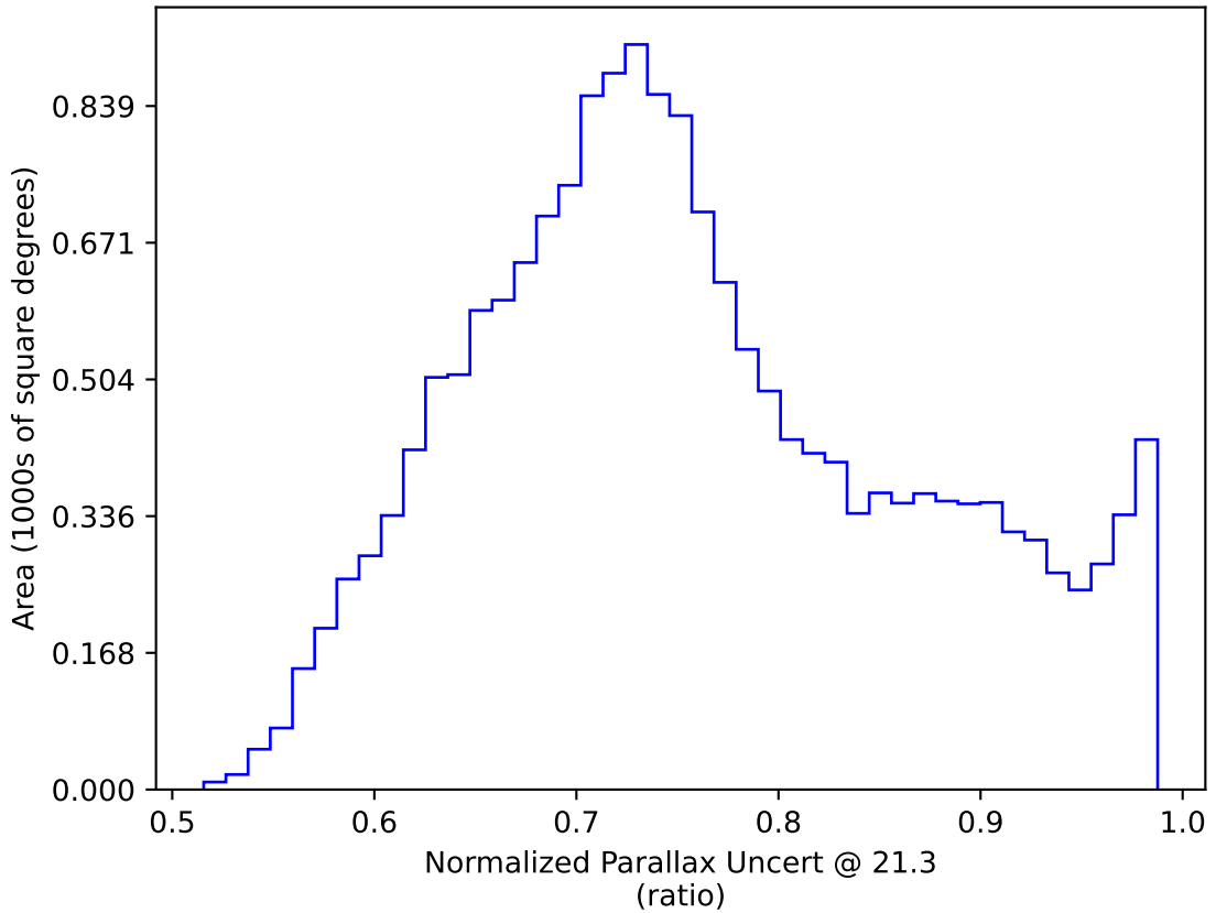
too_elab_heavy_r32_d2_griz_v3.4_10yrs WFD y band only: Normalized Parallax Uncert @ 21.3
