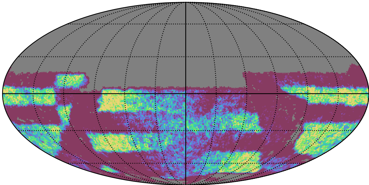
too_elab_heavy_r32_d2_griz_v3.4_10yrs Yr 3-4 y band: NVisits
