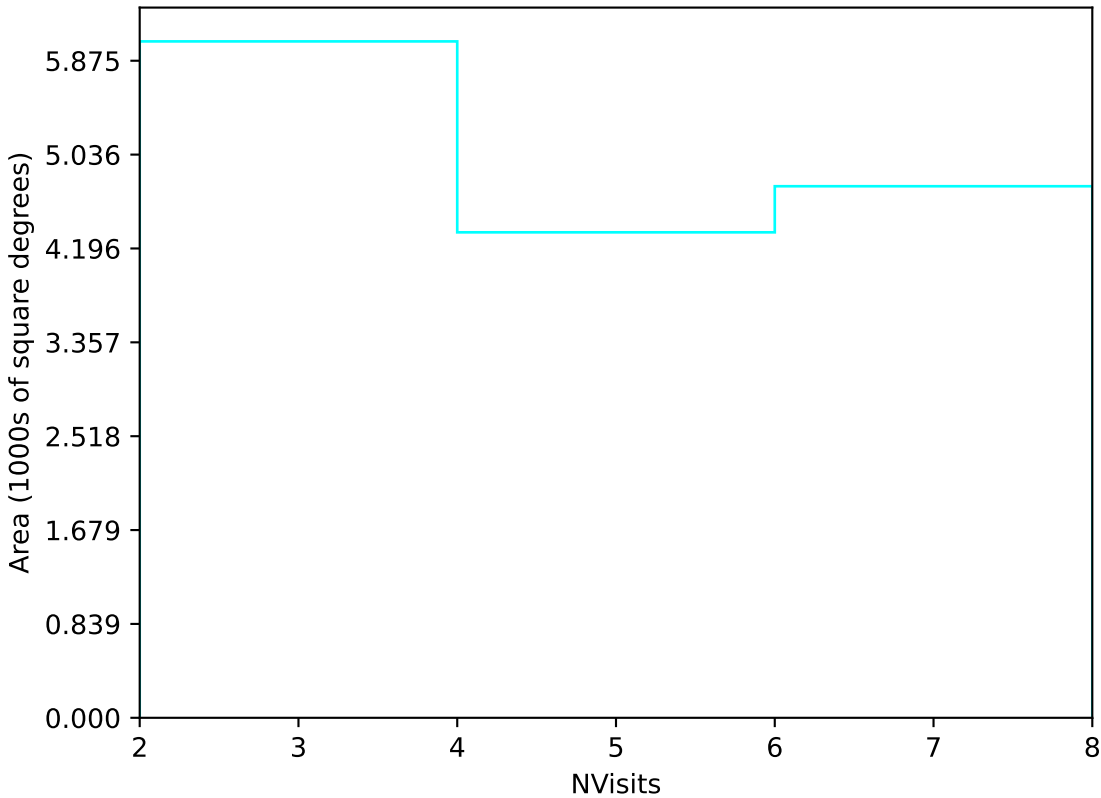
too_elab_heavy_r32_d2_griz_v3.4_10yrs Yr 3-4 u band: NVisits
