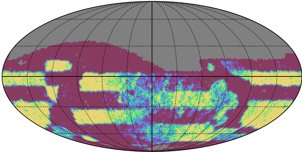
too_elab_heavy_r32_d2_griz_v3.4_10yrs Yr 3-4 r band: NVisits
