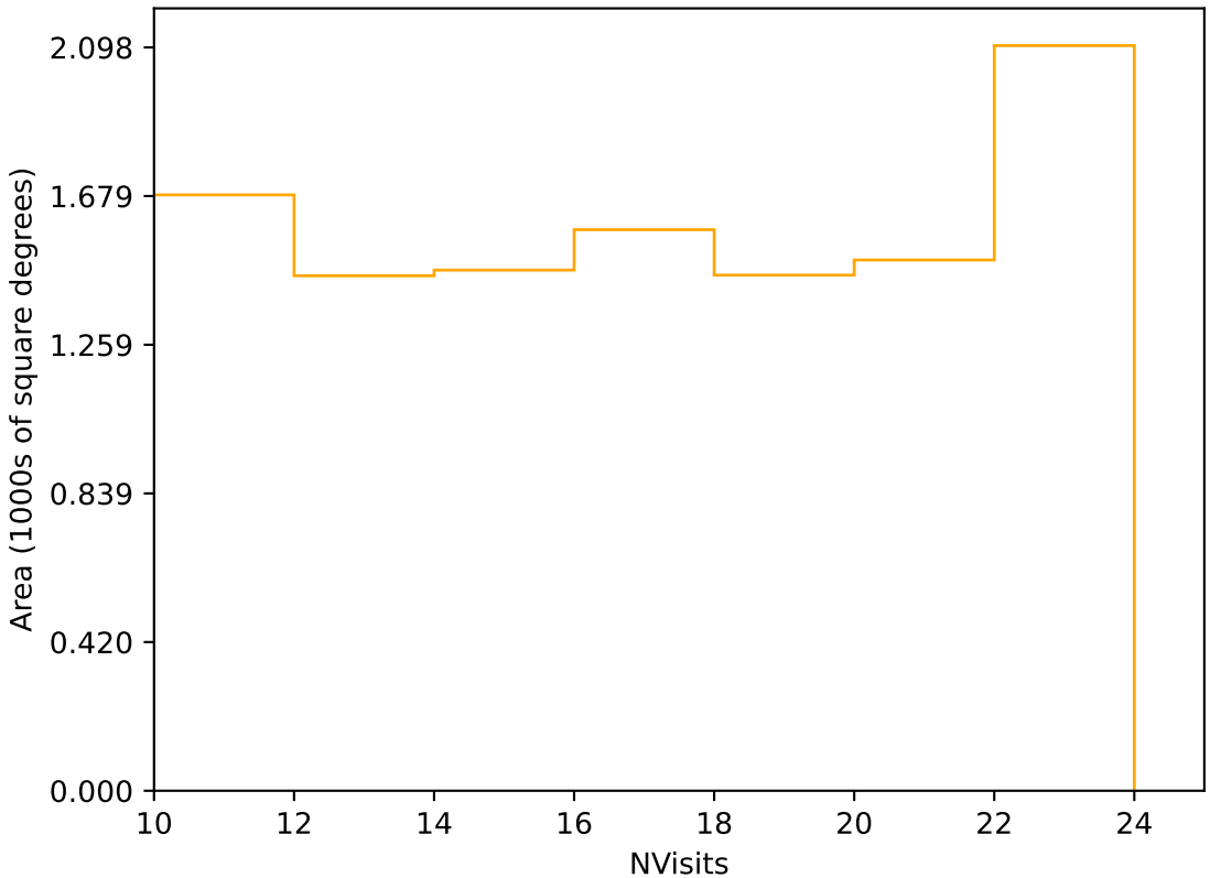
too_elab_heavy_r32_d2_griz_v3.4_10yrs Yr 3-4 r band: NVisits
