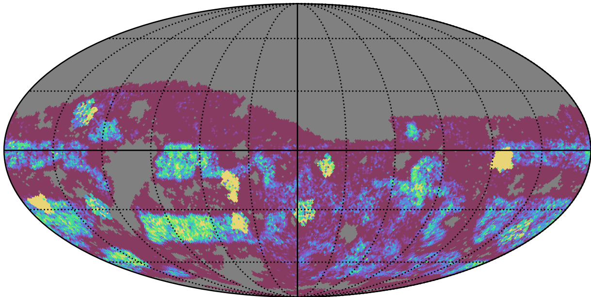
too_elab_heavy_r32_d2_griz_v3.4_10yrs Yr 3-4 g band: NVisits
