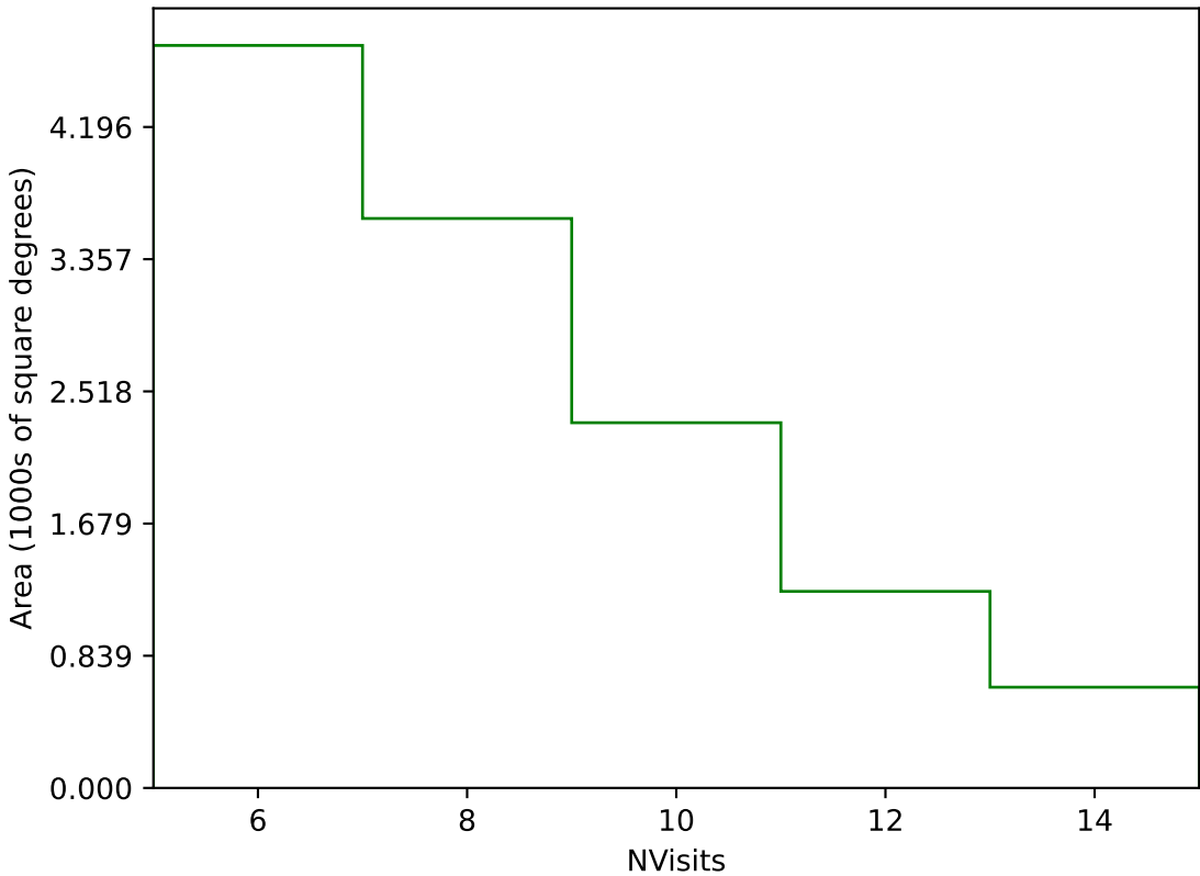
too_elab_heavy_r32_d2_griz_v3.4_10yrs Yr 3-4 g band: NVisits
