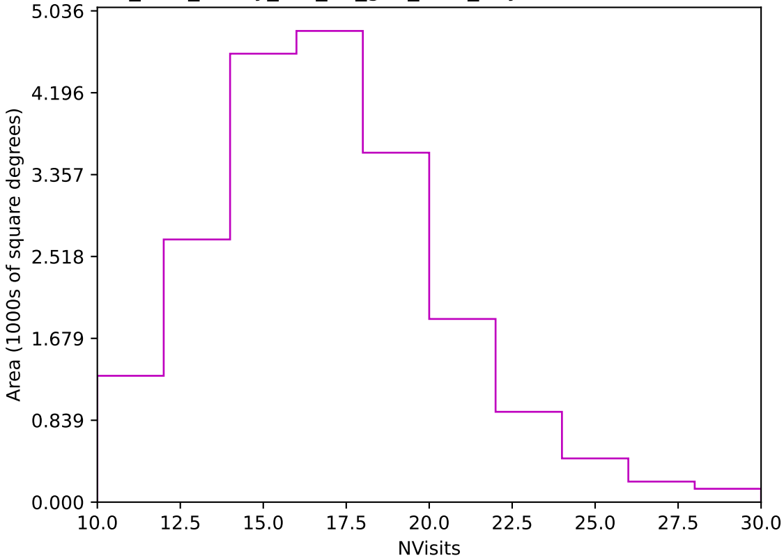
too_elab_heavy_r32_d2_griz_v3.4_10yrs Yr 1 z band: NVisits
