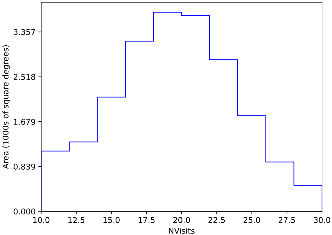
too_elab_heavy_r32_d2_griz_v3.4_10yrs Yr 1 y band: NVisits
