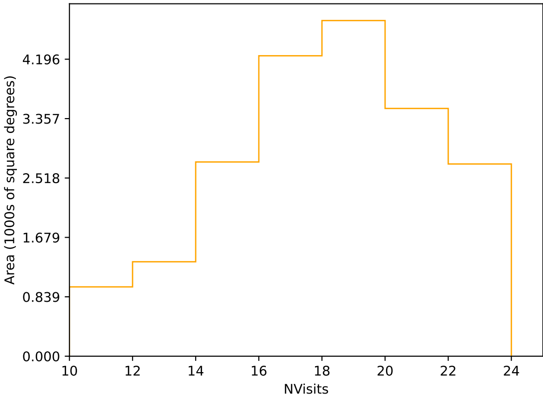
too_elab_heavy_r32_d2_griz_v3.4_10yrs Yr 1 r band: NVisits
