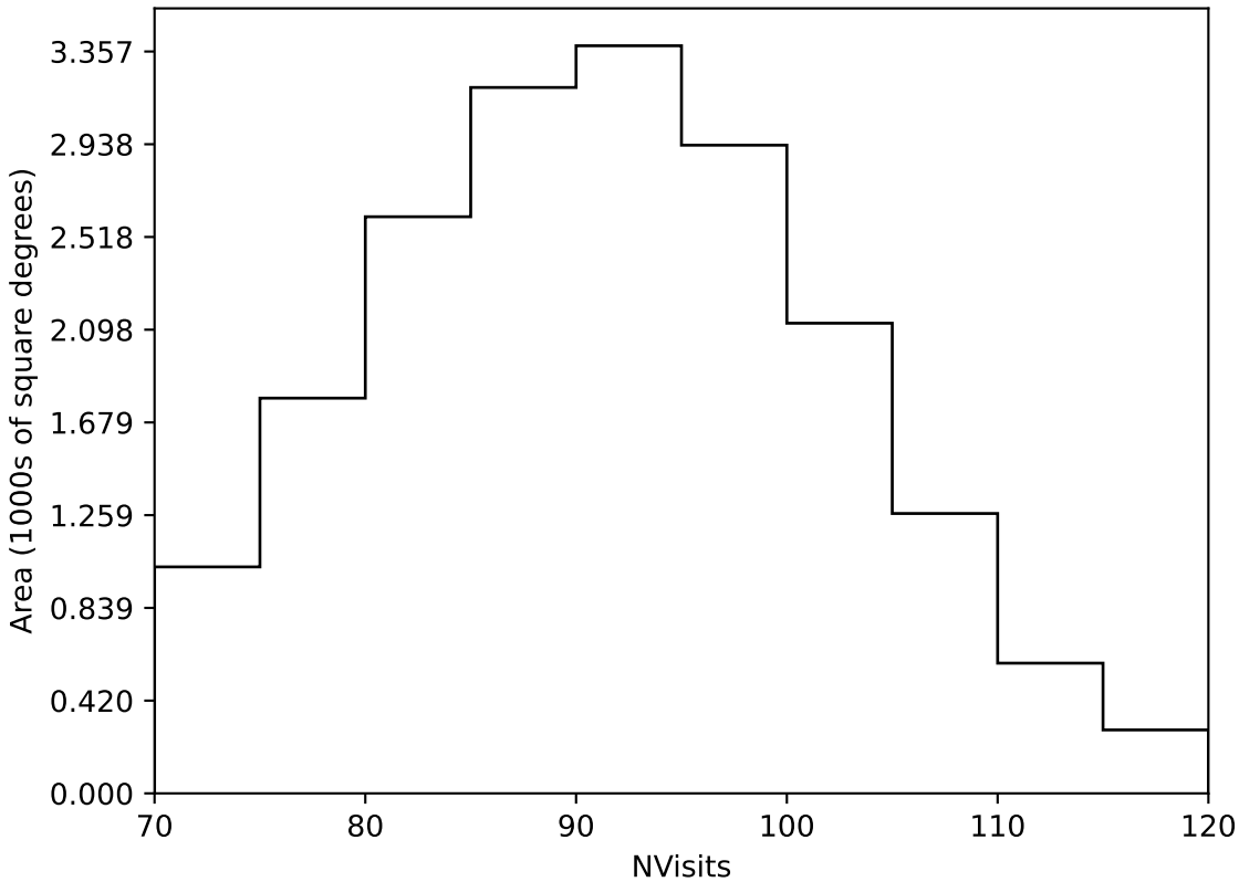
too_elab_heavy_r32_d2_griz_v3.4_10yrs Yr 1 all bands: NVisits
