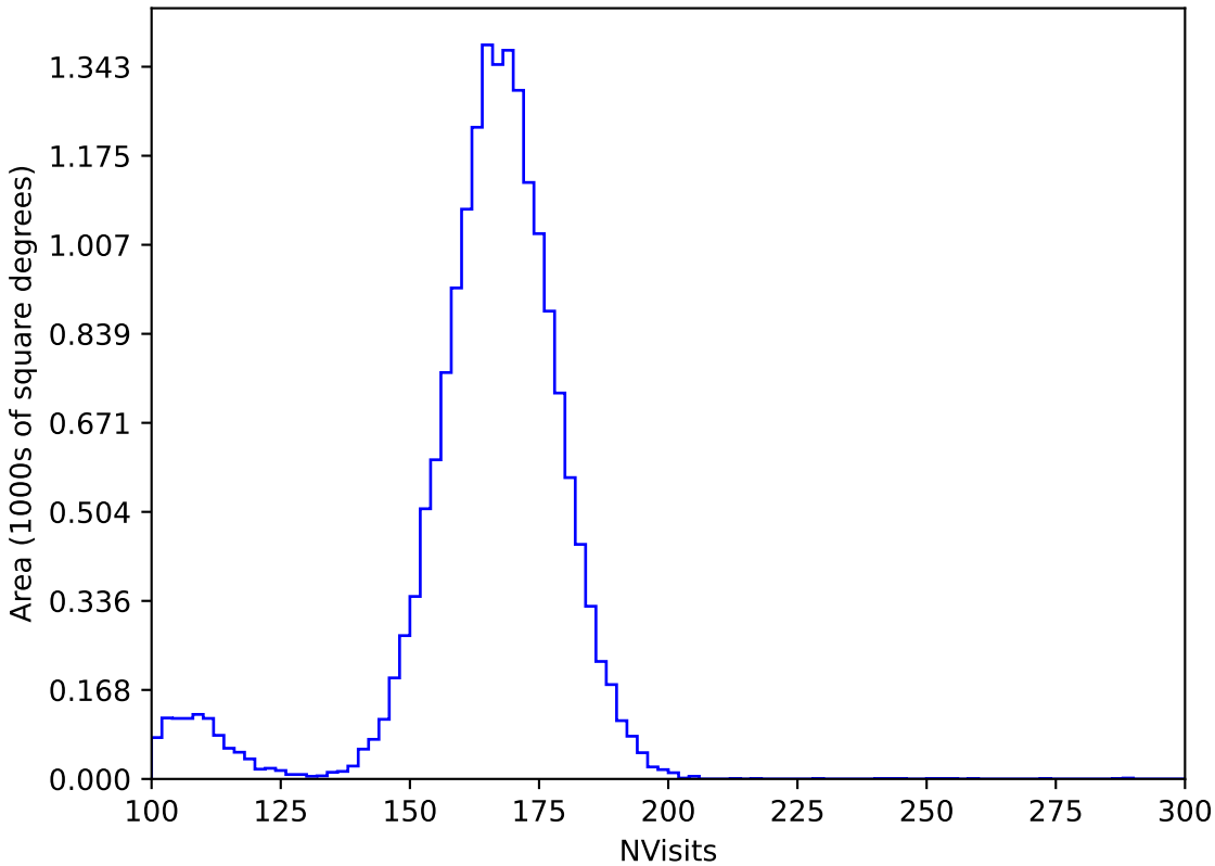
too_elab_heavy_r32_d2_griz_v3.4_10yrs WFD y band: NVisits
