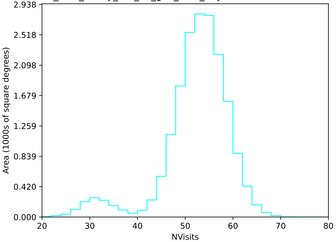
too_elab_heavy_r32_d2_griz_v3.4_10yrs WFD u band: NVisits
