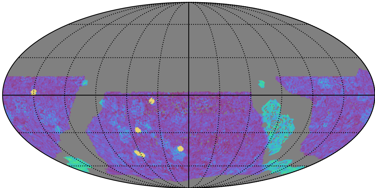
too_elab_heavy_r32_d2_griz_v3.4_10yrs WFD g band: NVisits
