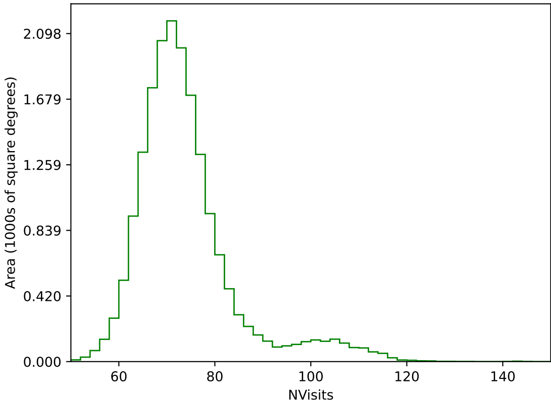
too_elab_heavy_r32_d2_griz_v3.4_10yrs WFD g band: NVisits
