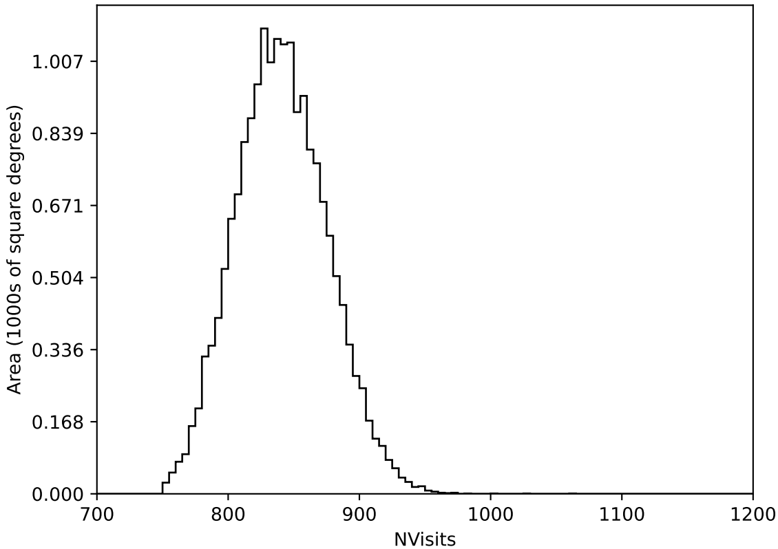
too_elab_heavy_r32_d2_griz_v3.4_10yrs WFD all bands: NVisits
