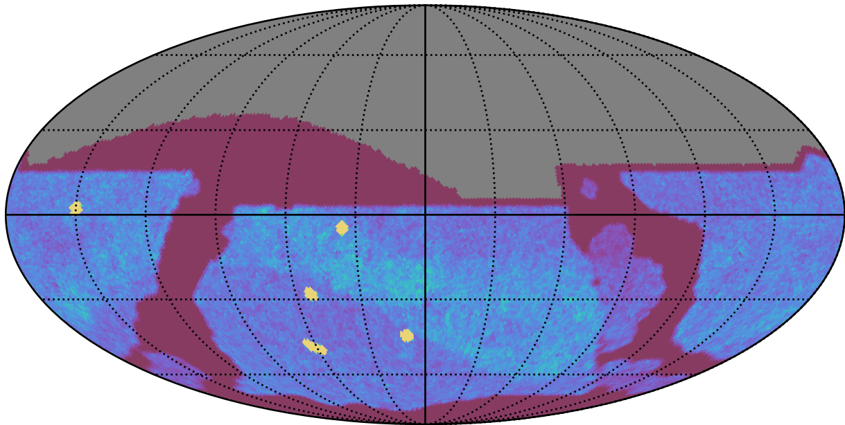
too_elab_heavy_r32_d2_griz_v3.4_10yrs All sky z band: NVisits
