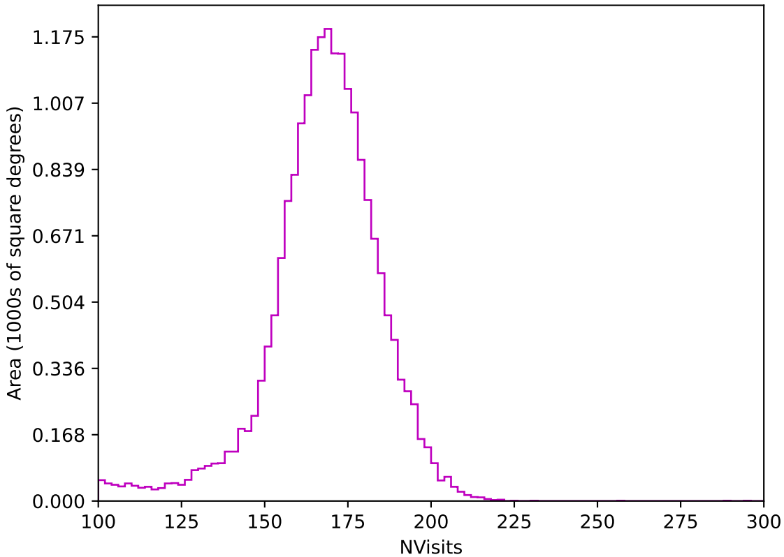
too_elab_heavy_r32_d2_griz_v3.4_10yrs All sky z band: NVisits
