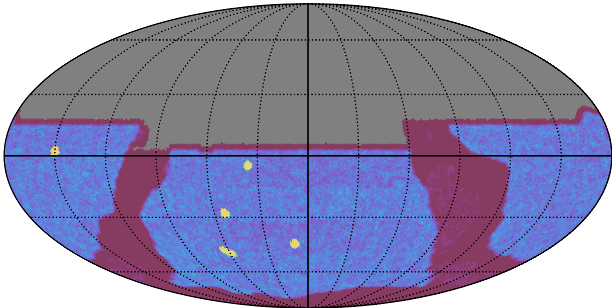
too_elab_heavy_r32_d2_griz_v3.4_10yrs All sky y band: NVisits
