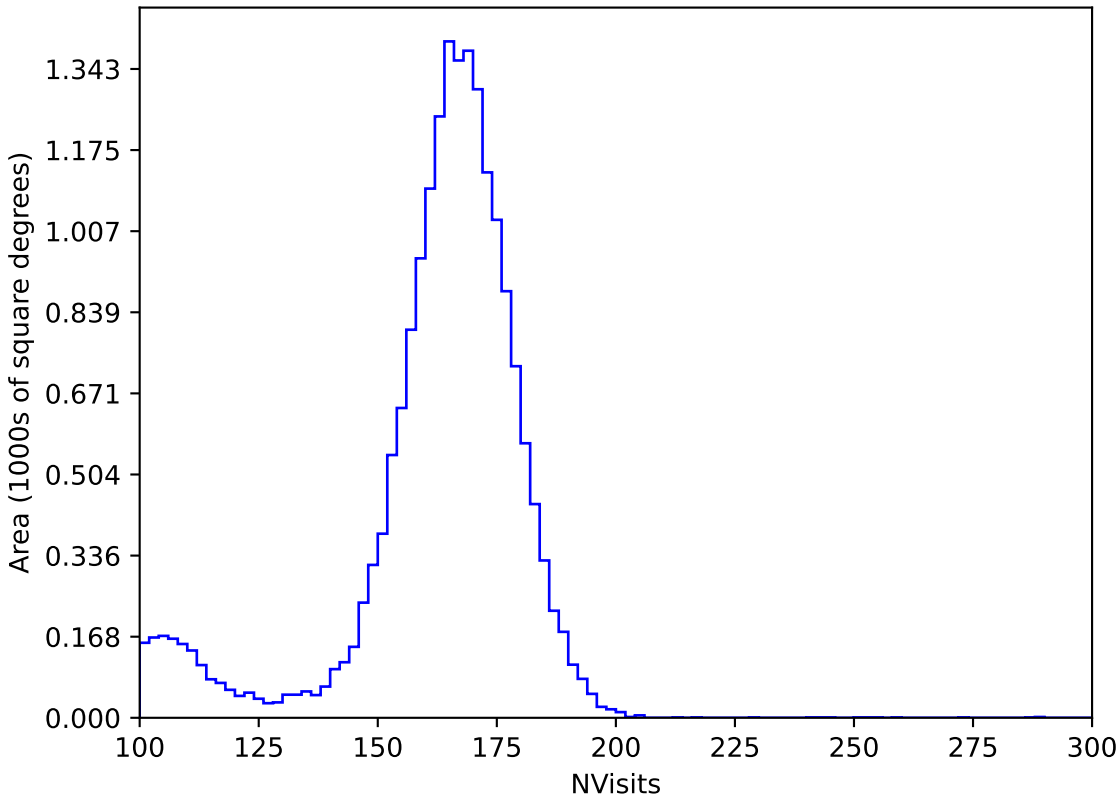
too_elab_heavy_r32_d2_griz_v3.4_10yrs All sky y band: NVisits
