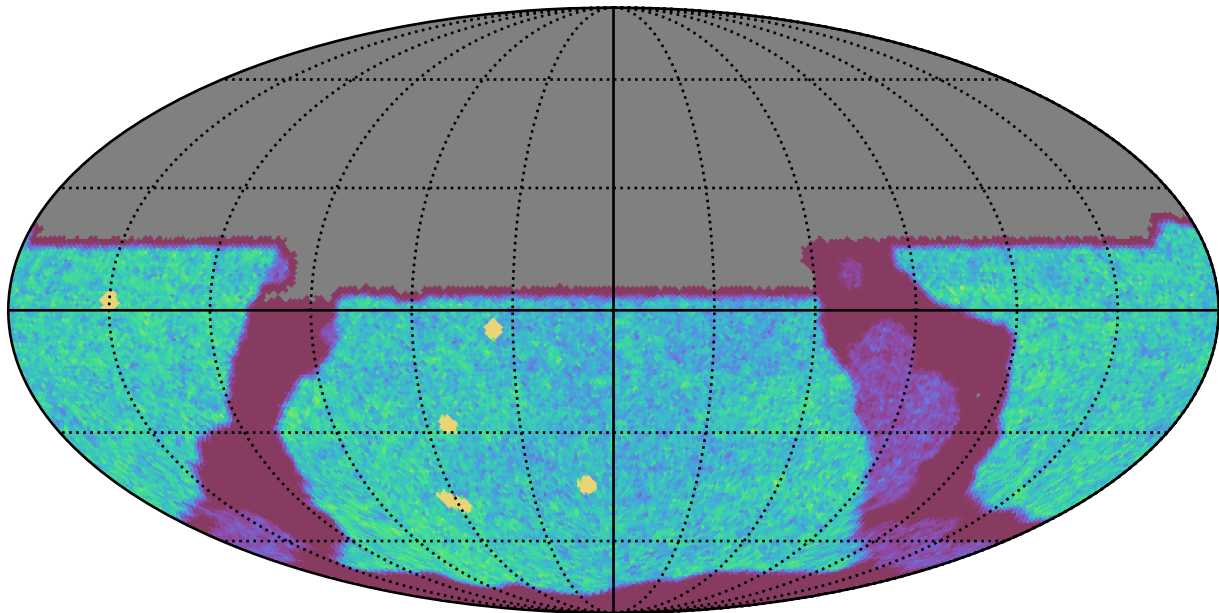
too_elab_heavy_r32_d2_griz_v3.4_10yrs All sky u band: NVisits
