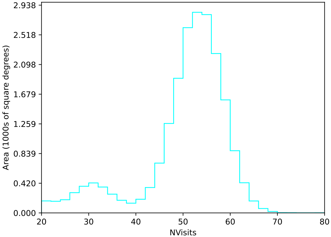
too_elab_heavy_r32_d2_griz_v3.4_10yrs All sky u band: NVisits
