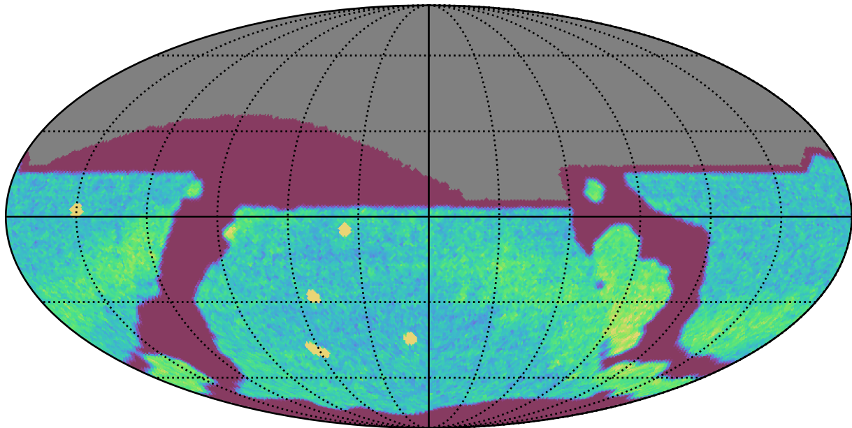
too_elab_heavy_r32_d2_griz_v3.4_10yrs All sky r band: NVisits
