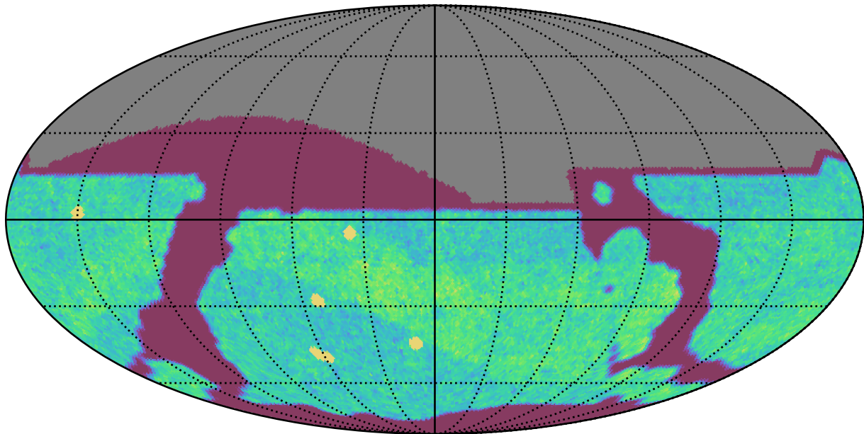
too_elab_heavy_r32_d2_griz_v3.4_10yrs All sky i band: NVisits
