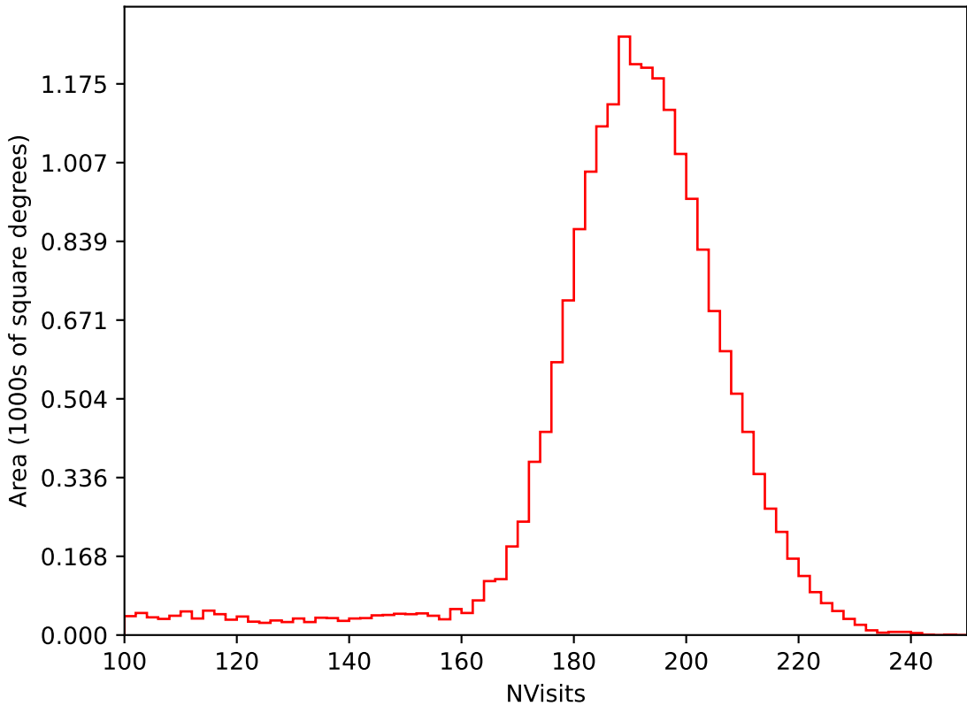
too_elab_heavy_r32_d2_griz_v3.4_10yrs All sky i band: NVisits
