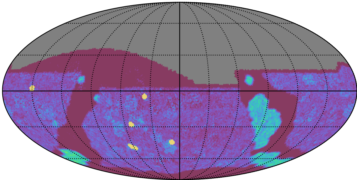
too_elab_heavy_r32_d2_griz_v3.4_10yrs All sky g band: NVisits
