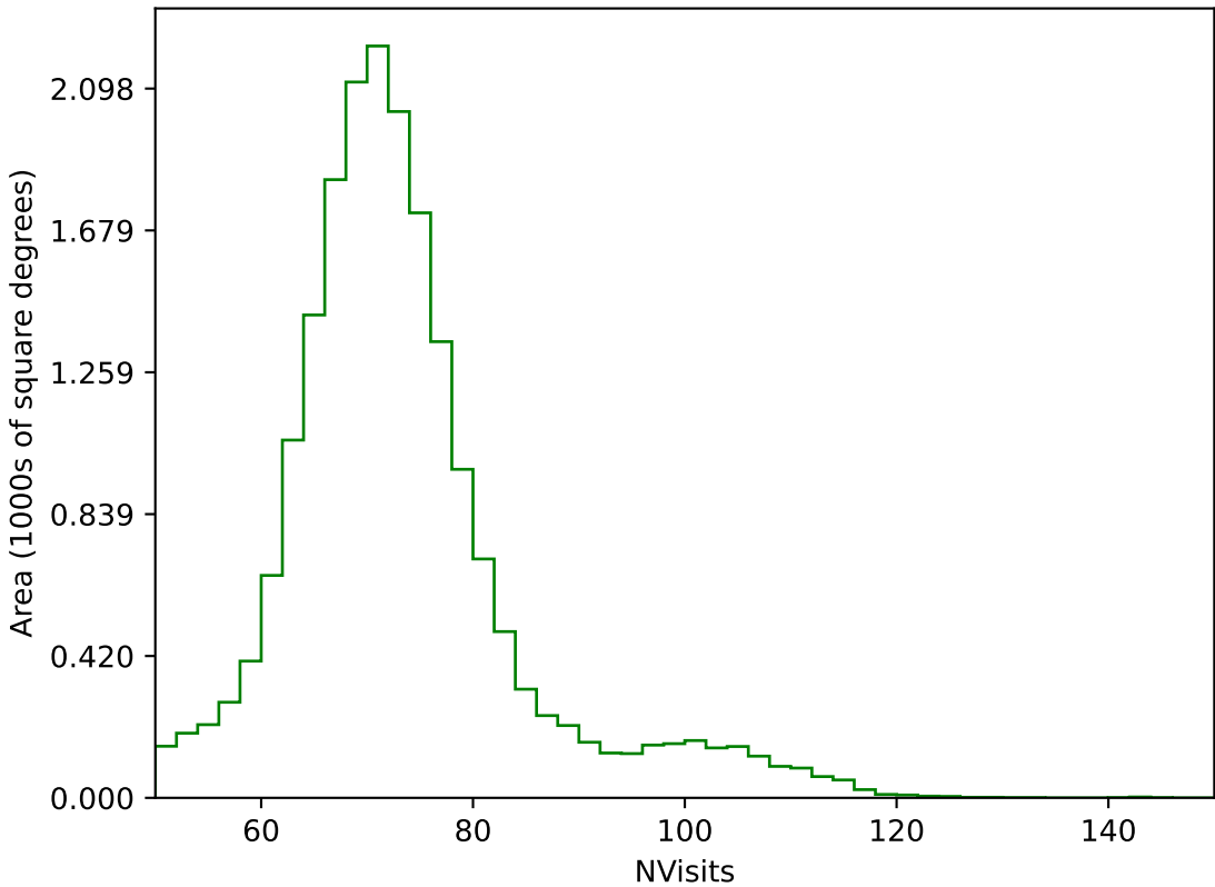
too_elab_heavy_r32_d2_griz_v3.4_10yrs All sky g band: NVisits
