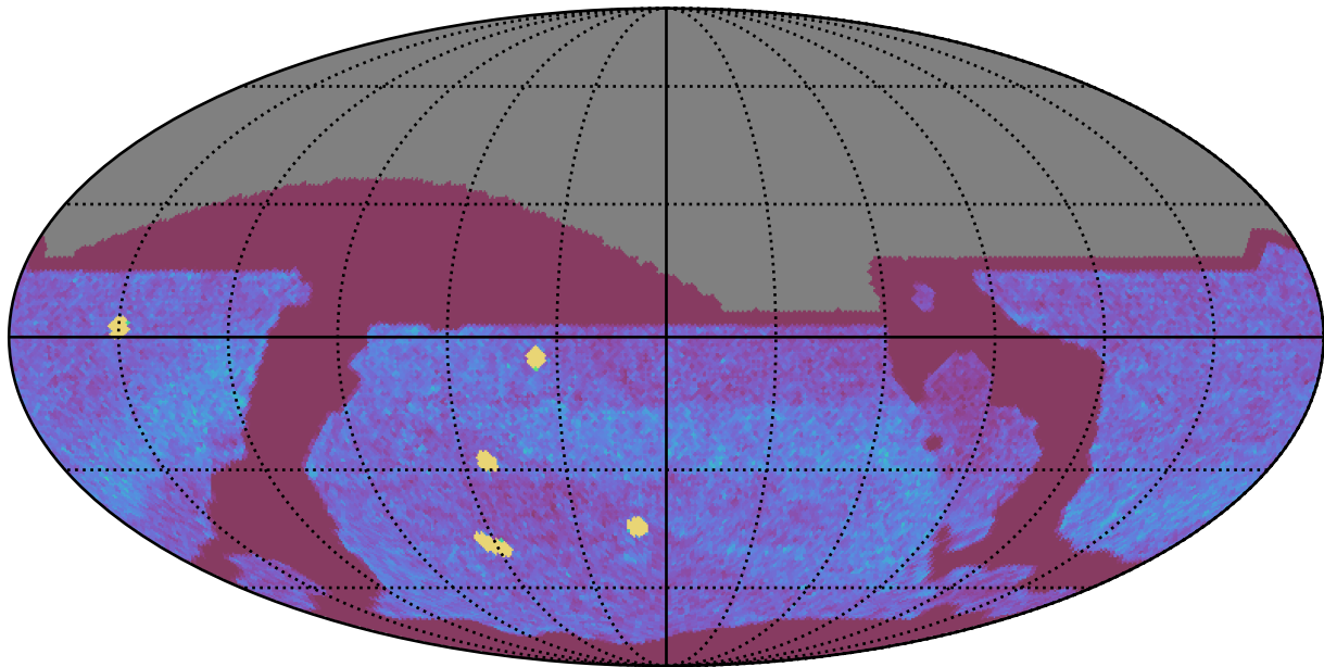
too_elab_heavy_r32_d2_griz_v3.4_10yrs All sky all bands: NVisits
