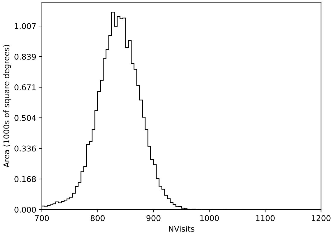
too_elab_heavy_r32_d2_griz_v3.4_10yrs All sky all bands: NVisits
