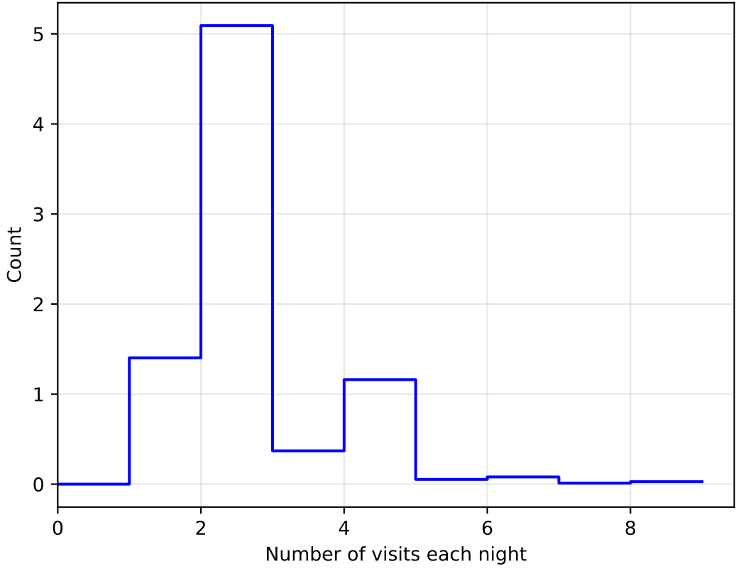
too_elab_heavy_r32_d2_griz_v3.4_10yrs WFD: NVisitsPerNight 1e6
