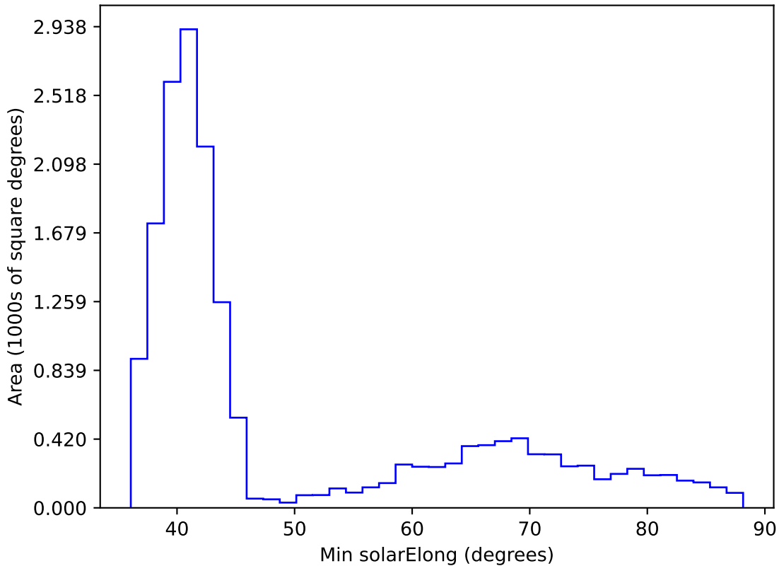
too_elab_heavy_r32_d2_griz_v3.4_10yrs WFD i band: Min solarElong
