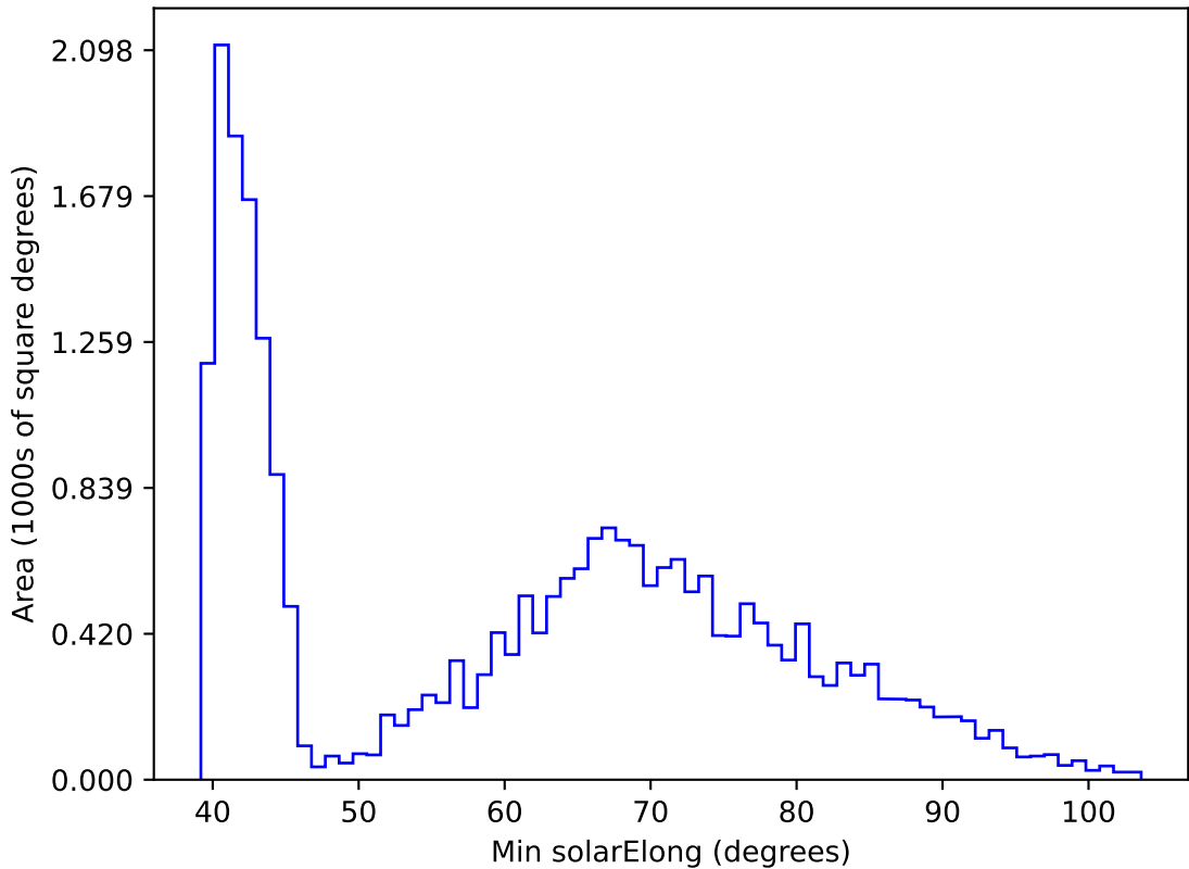
too_elab_heavy_r32_d2_griz_v3.4_10yrs All sky r band: Min solarElong
