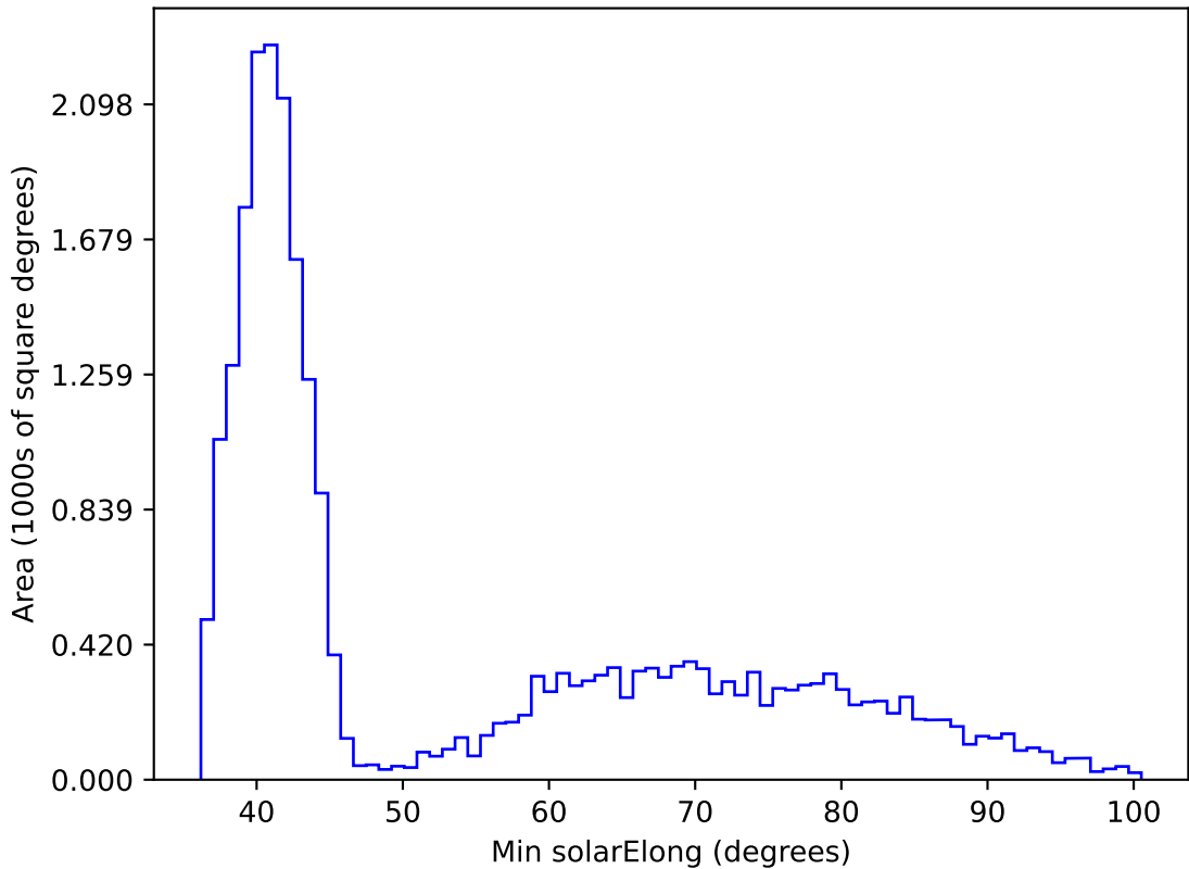
too_elab_heavy_r32_d2_griz_v3.4_10yrs All sky i band: Min solarElong
