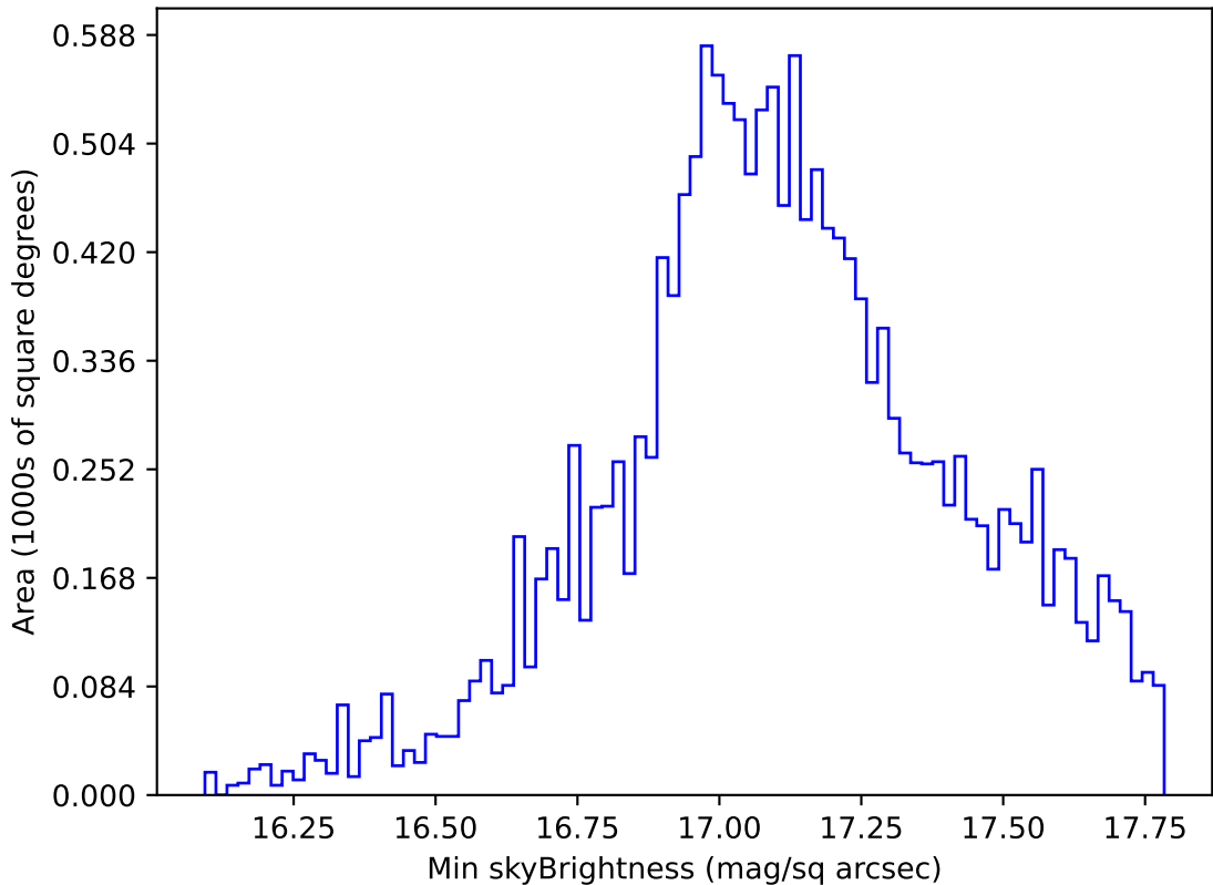
too_elab_heavy_r32_d2_griz_v3.4_10yrs WFD y band: Min skyBrightness
