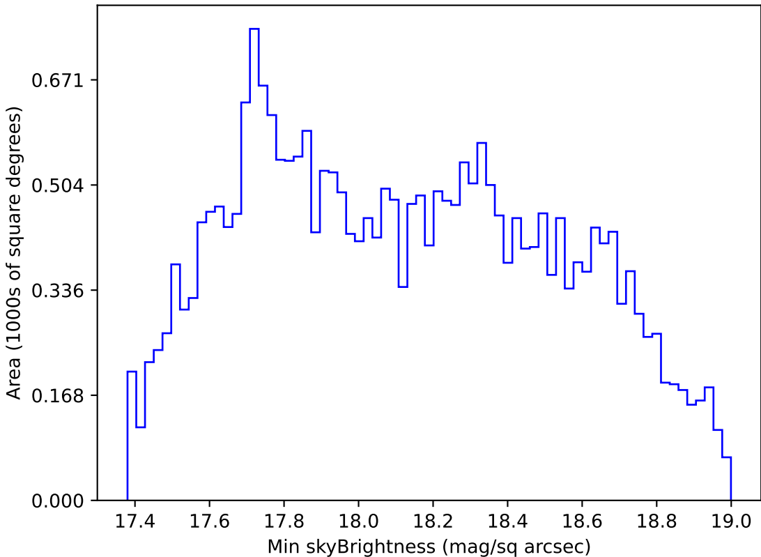
too_elab_heavy_r32_d2_griz_v3.4_10yrs All sky i band: Min skyBrightness
