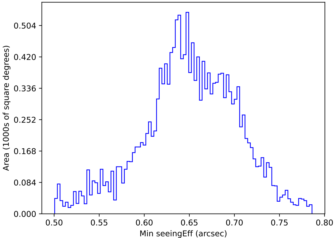
too_elab_heavy_r32_d2_griz_v3.4_10yrs WFD g band: Min seeingEff
