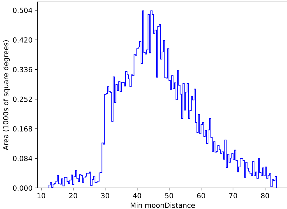
too_elab_heavy_r32_d2_griz_v3.4_10yrs All sky g band: Min moonDistance
