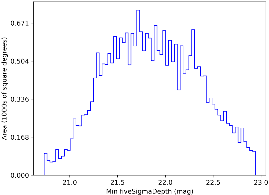
too_elab_heavy_r32_d2_griz_v3.4_10yrs All sky i band: Min fiveSigmaDepth
