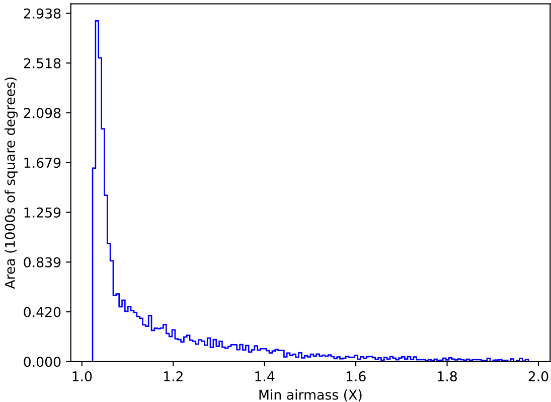
too_elab_heavy_r32_d2_griz_v3.4_10yrs Yr 1 i band: Min airmass
