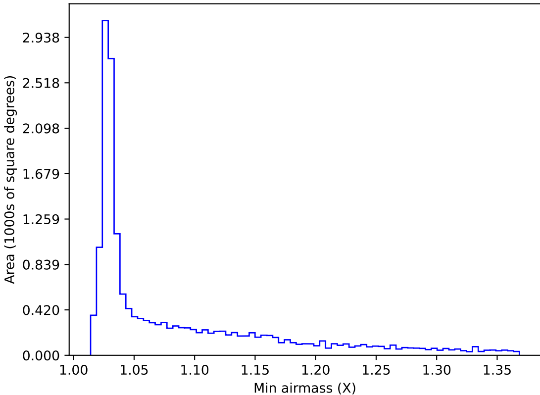
too_elab_heavy_r32_d2_griz_v3.4_10yrs WFD z band: Min airmass
