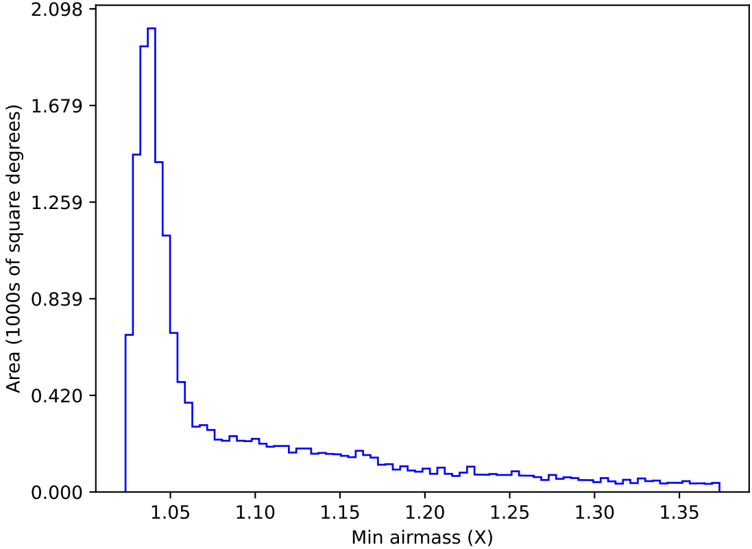
too_elab_heavy_r32_d2_griz_v3.4_10yrs WFD u band: Min airmass
