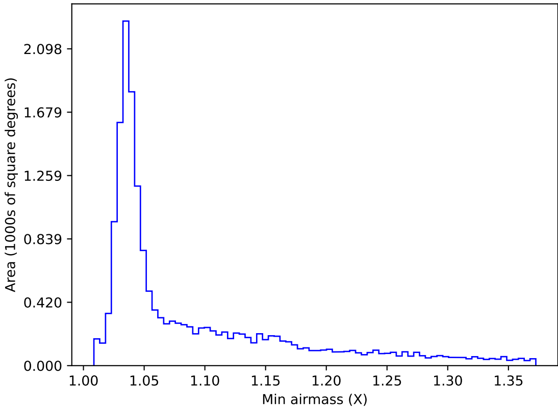
too_elab_heavy_r32_d2_griz_v3.4_10yrs WFD g band: Min airmass
