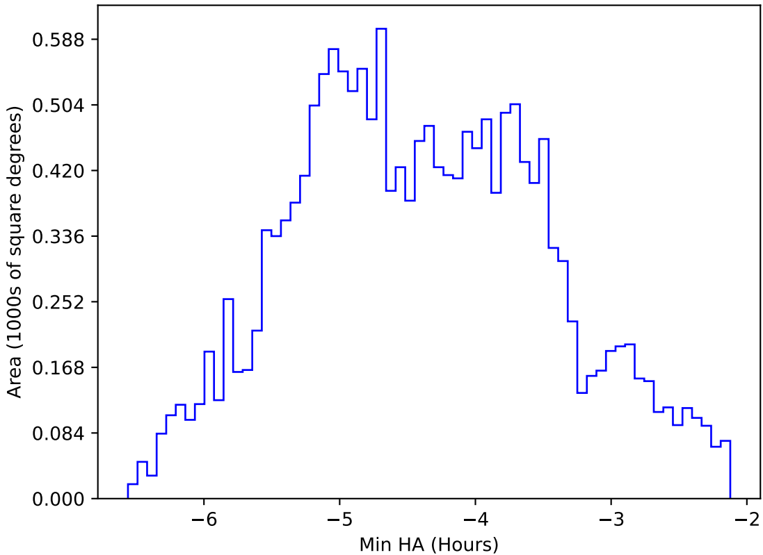
too_elab_heavy_r32_d2_griz_v3.4_10yrs WFD z band: Min HA
