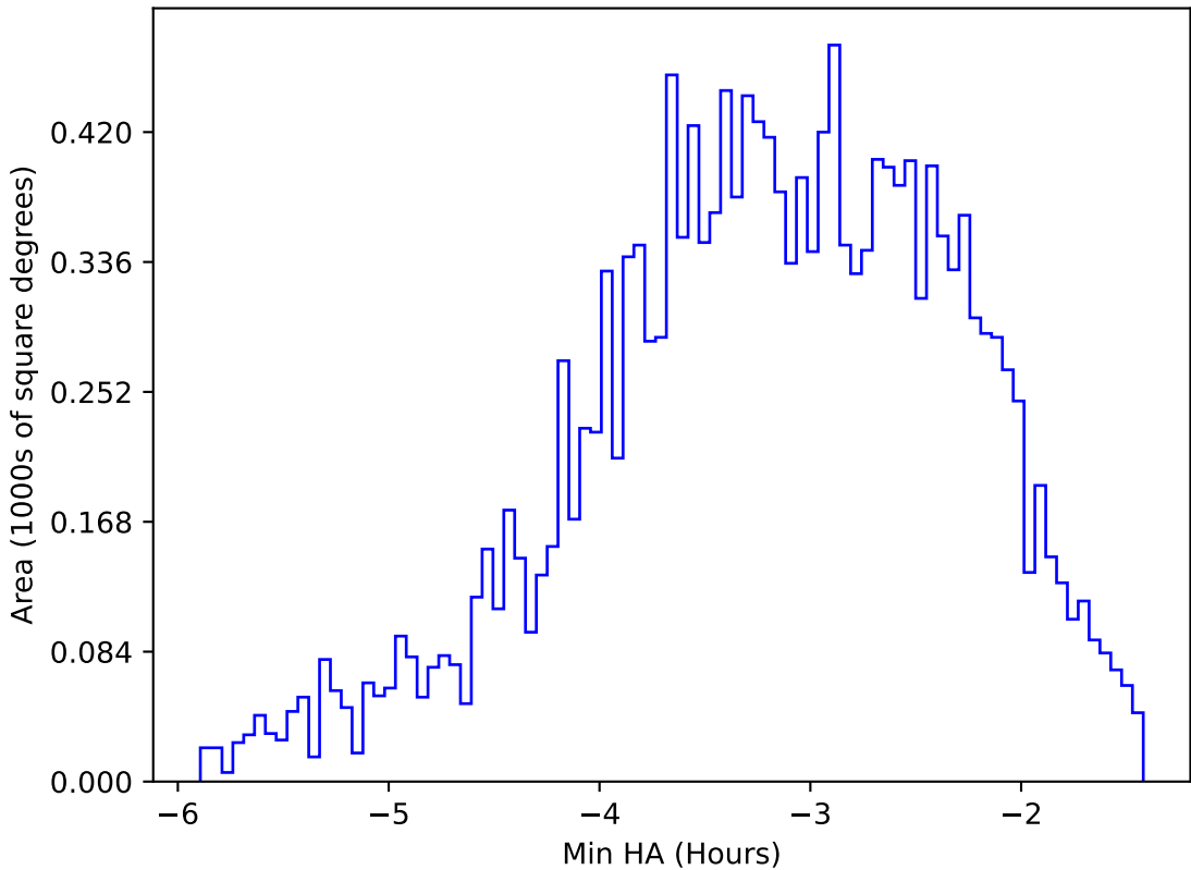
too_elab_heavy_r32_d2_griz_v3.4_10yrs WFD u band: Min HA
