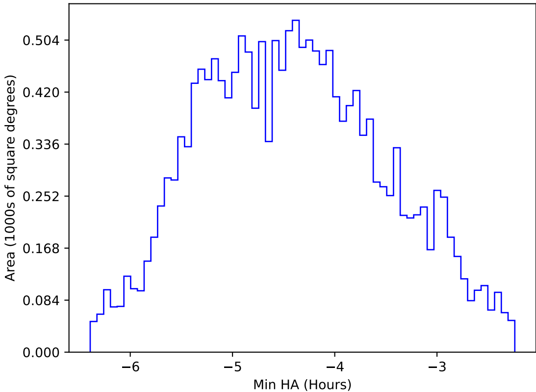
too_elab_heavy_r32_d2_griz_v3.4_10yrs WFD r band: Min HA
