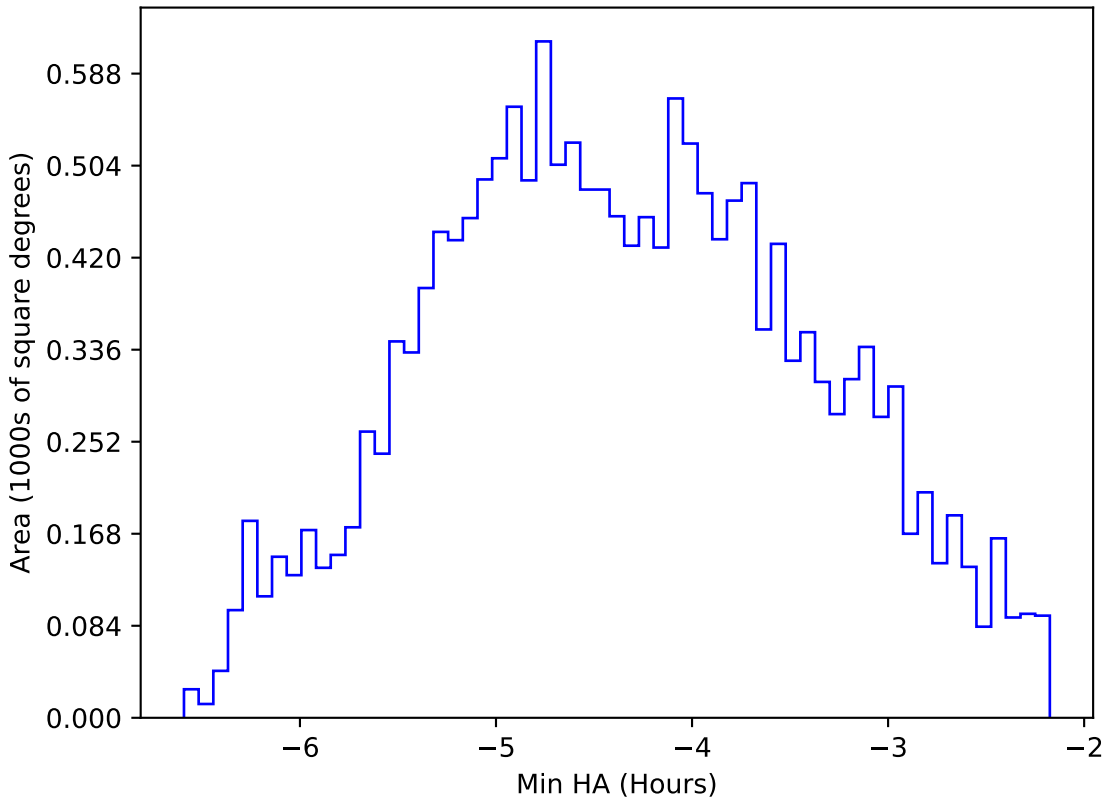
too_elab_heavy_r32_d2_griz_v3.4_10yrs WFD i band: Min HA
